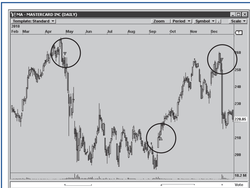
Signals on MA from the Breakout (Stocks) DO Strategy. The Strategy tends to find the most powerful Breakouts.
